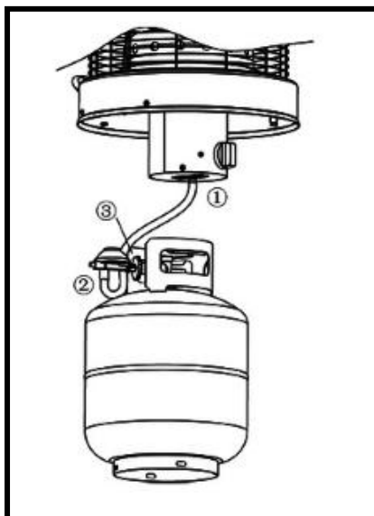
Leak Test Point ① ② ③
